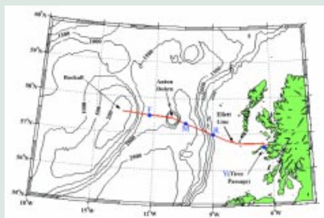
Fig. 29 Chart showing the position of the Ellett Line to the west of Scotland.
