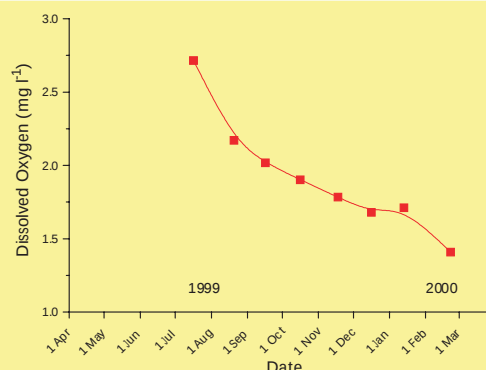
Fig. 43 Changes in oxygen concentration below 80 m depth from July 1999 – February 2000 in the deep basin, Loch Etive.
