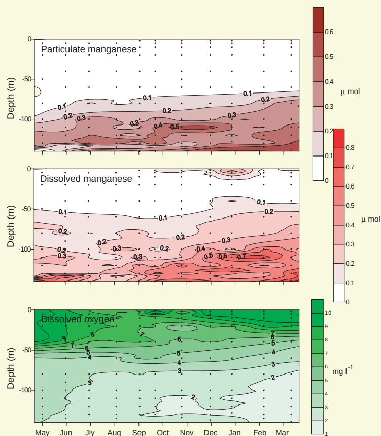
Fig. 44 Contour plots of particulate and dissolved manganese and of dissolved oxygen versus depth as a function of time at the deep station in the upper basin of Loch Etive (140 m). The dots mark the positions of the individual samples.
