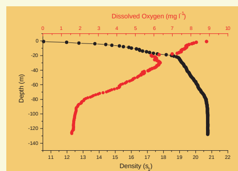
Fig. 41 Strong density stratification in the deep basin of Loch Etive in October 1999 and an oxycline from 30 to 80 m depth.
