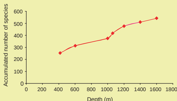
Fig. 9 Accumulation of previously unrecorded macrobenthic species in box cores on the Hebridean slope. The samples are assembled along the depth gradient and show a sharp, step-like increase in rate of accumulation at about 1000-1200 m, indicating a marked change in community composition at about this depth.
