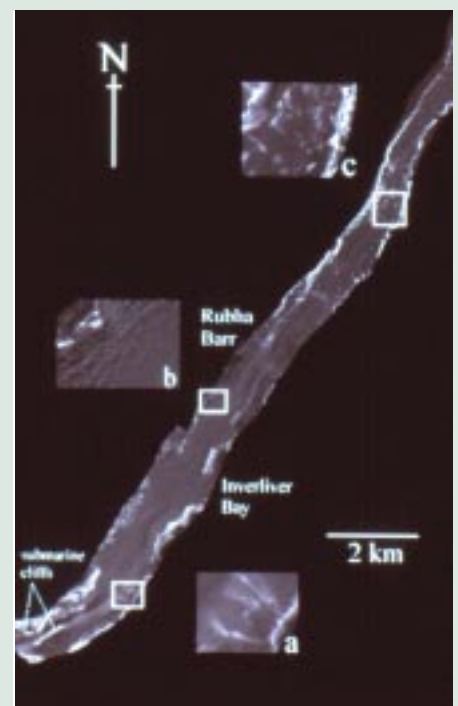
Fig. 26 Side-scan sonar survey of upper Loch Etive. Insets: (a) Outwash fans from the River Noe; (b) Sediment creep, due to gravity-induced mass wasting of water-laden soft sediment on the steep slopes; (c) Boulders on the loch floor, possibly a result of glacial retreat or post glacial rockfall.
