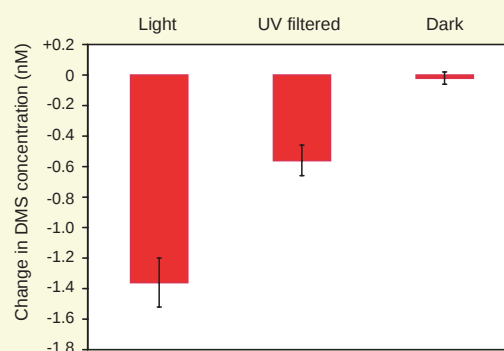
Fig. 23 The average change in DMS concentration in samples incubated for eight hours under light, UV filtered and dark conditions. Results clearly show light-dependent removal of DMS.
