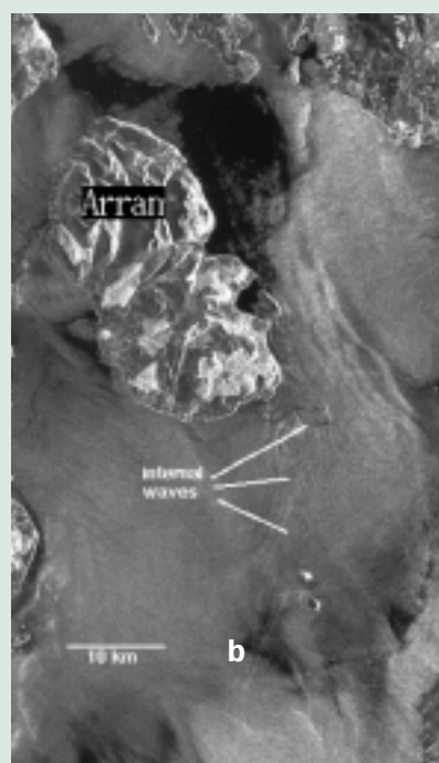
Fig. 27 Synthetic Aperture Radar Image of the southern Firth of Clyde from the ERS2 satellite. The light and dark bands indicated are the surface manifestation of internal waves generated by the submarine sill which runs from Arran to Ailsa Craig. Feature b is the internal wake of the Seacat ferry. The image size is 30 km by 30 km and was kindly provided by the Defence Evaluation and Research Agency, Farnborough.
