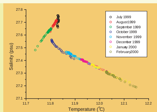
Fig. 42 Temperature and salinity changes in the deep basin of Loch Etive from July 1999 – February 2000.
