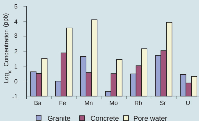
Fig. 38 A comparison of heavy metal levels derived from granite, sea loch sediment pore waters and the concrete blocks intended for deployment in the experimental artificial reef.
