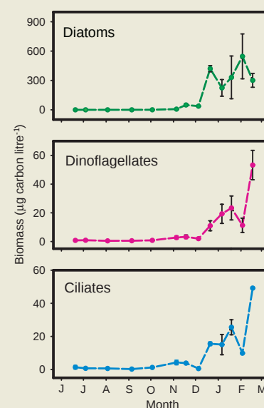
Fig. 18 Microplankton biomass in Ryder Bay, Antarctica.
