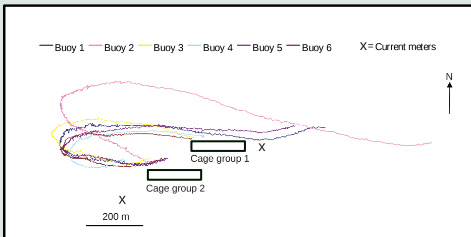
Fig. 46 Drifter buoy survey on 6 March in Loch Sunart, with positions of current meters and cage groups. Release started at 11:45, tide turned at 13:30, release ended at 15:45.
