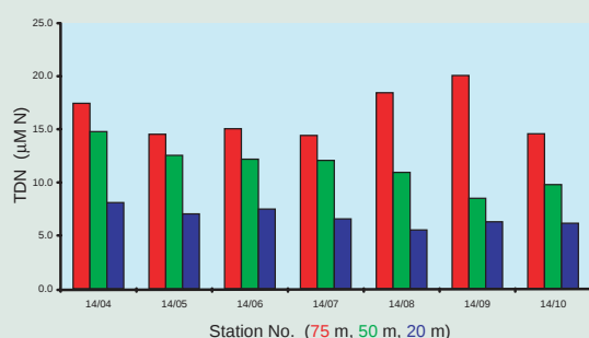
Fig. 30 Concentrations of total dissolved nitrogen (TDN) and dissolved organic nitrogen (DON) where TDN=DON, at seven stations along an oceanic transect in the northern North Sea, on 14th June 1999. Concentrations of inorganic nitrogen nutrients were in the nano-molar region at all depths for all stations.
