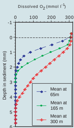
Fig. 3 Interstitial dissolved oxygen profiles from the Beryl "A" cuttings pile showing an increase in oxygen penetration with distance from the platform. The dashed line at 0-mm depth marks the position of the sediment-water interface.
