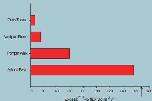
Fig. 4 Excess ^{210}\text{Pb} fluxes for all four stations studied. Arrow indicates calculated mean of global flux.
