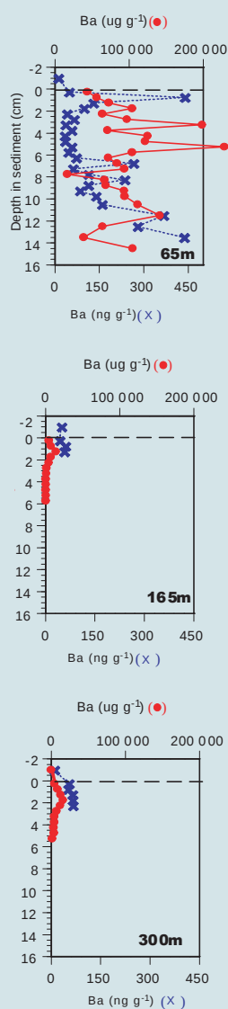
Fig. 2 Interstitial dissolved (x) and solid phase (●) barium concentrations measured in the sediments at three distances from an oil production platform. Barium contamination declines markedly with increasing distance from the drilling site. The dashed line represents the sediment-water interface.
