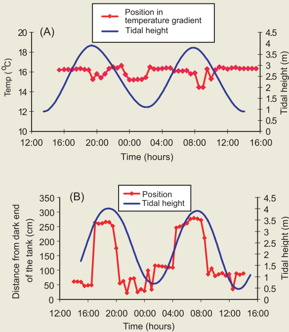
Fig. 35 Positions selected by juvenile turbot within (A) temperature and (B) light gradients.
