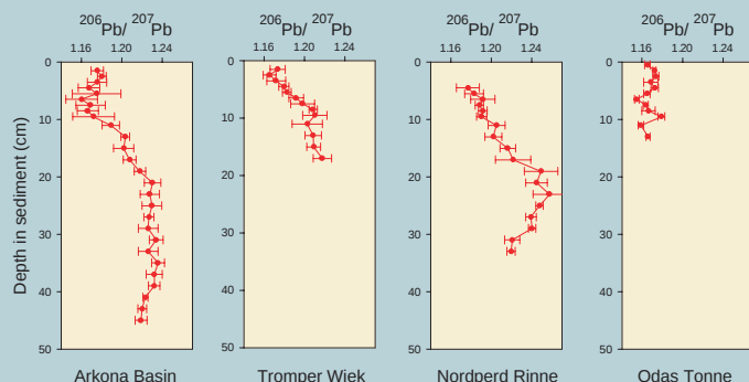
Fig. 5 Lead isotope profiles for Baltic Sea sediment cores.
