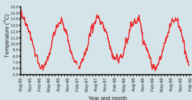
Fig. 36 A 5-year subtidal seawater temperature profile obtained from submerged autonomous temperature loggers. Each value is a daily average of 120 measurements.
