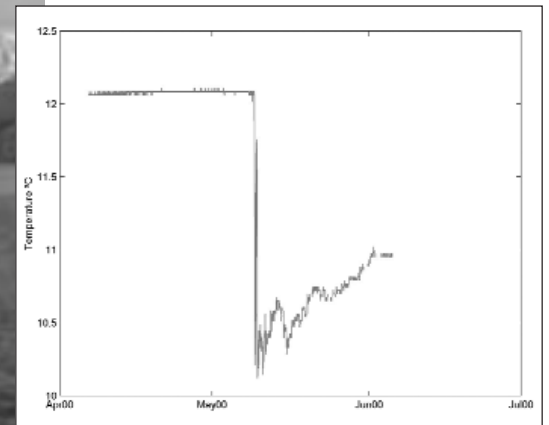
Deep water in Loch Etive had been isolated from the open sea since at least the summer of 1999. Renewal is indicated by an abrupt temperature decrease on 11 May 2000.
